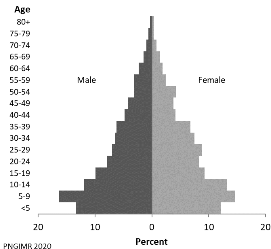
Figure 2. Population pyramid
