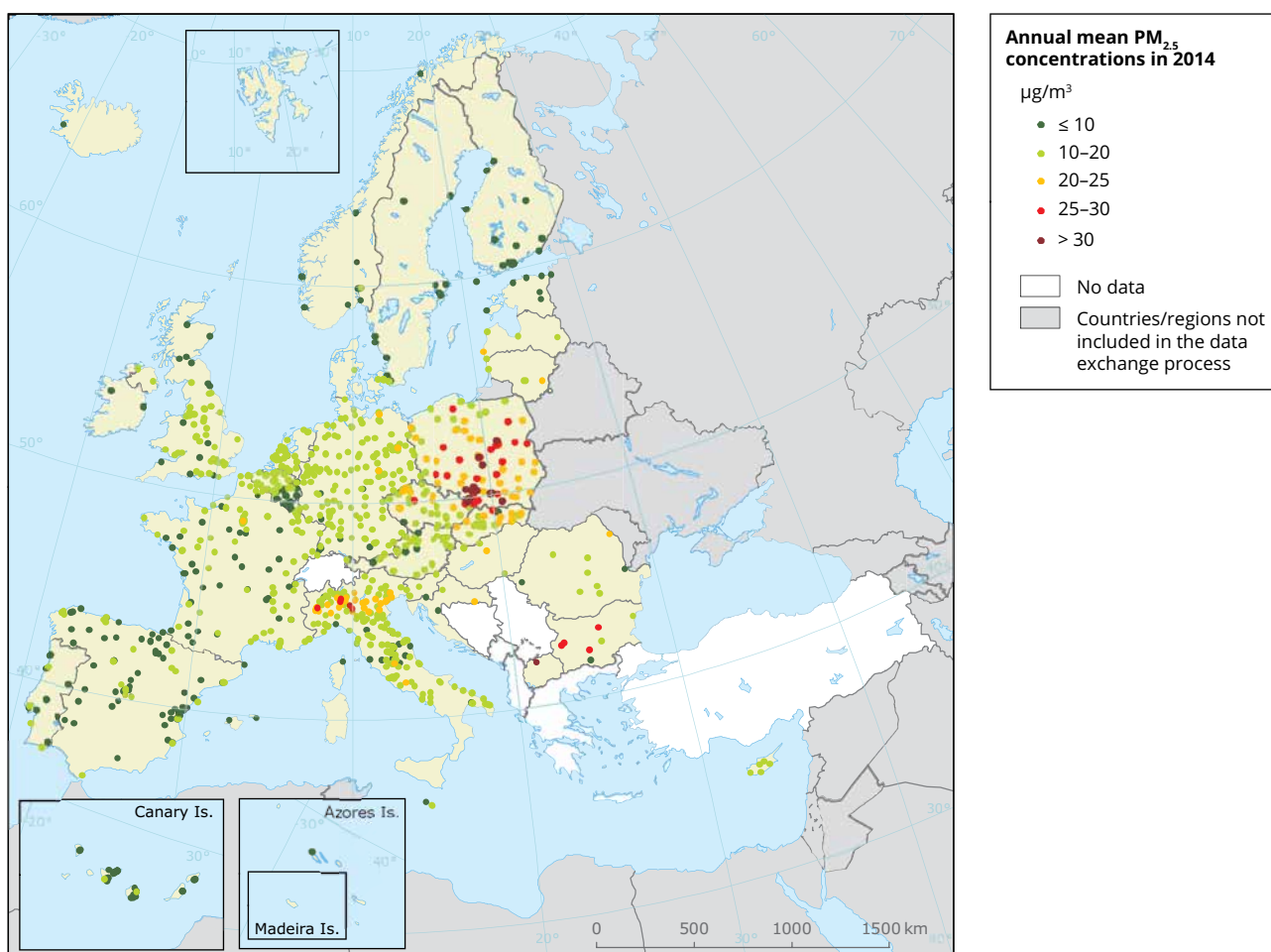
Map 4.2 Concentrations of PM_{2.5} in 2014
