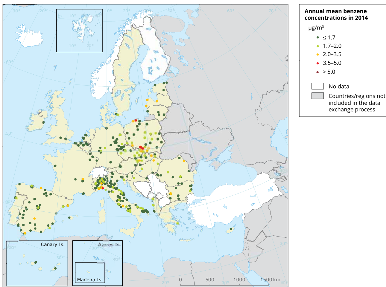
Map 8.3 Concentrations of benzene in 2014
