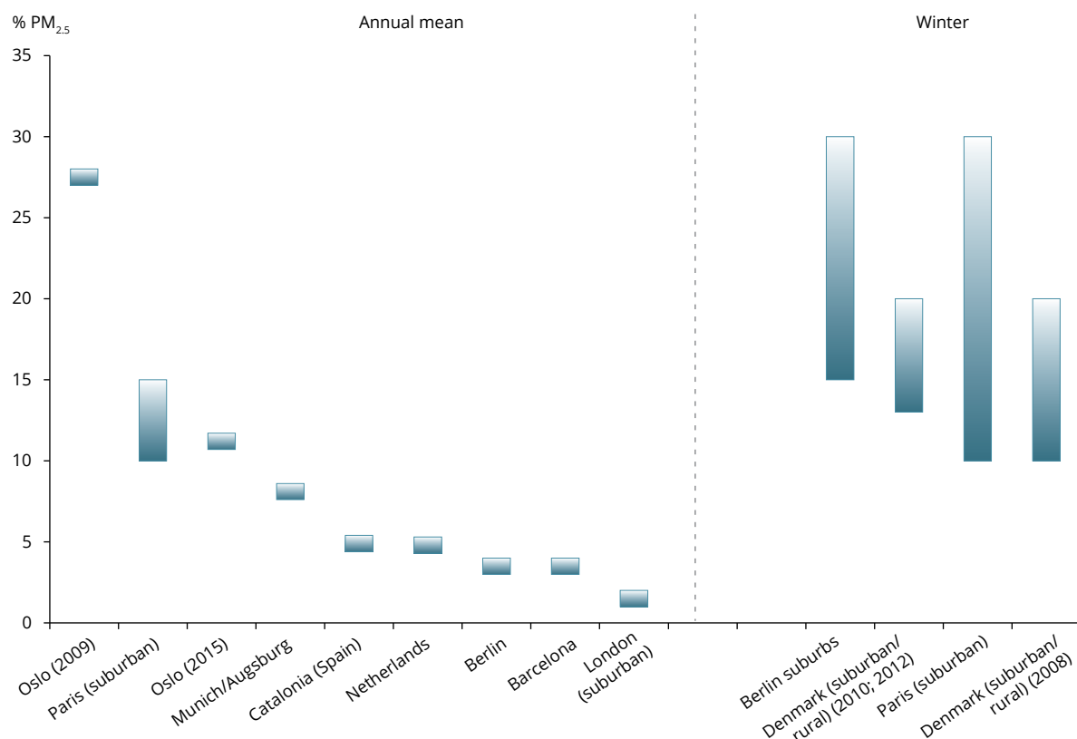
Figure 3.2 Studies quantifying the impact of residential combustion on PM 2.5
