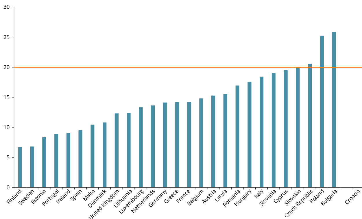
Figure 9.1 Urban and suburban background PM 2.5 concentrations presented as 3-year averages in the EU-28 (2012–2014), as an approximation of the average exposure indicator
