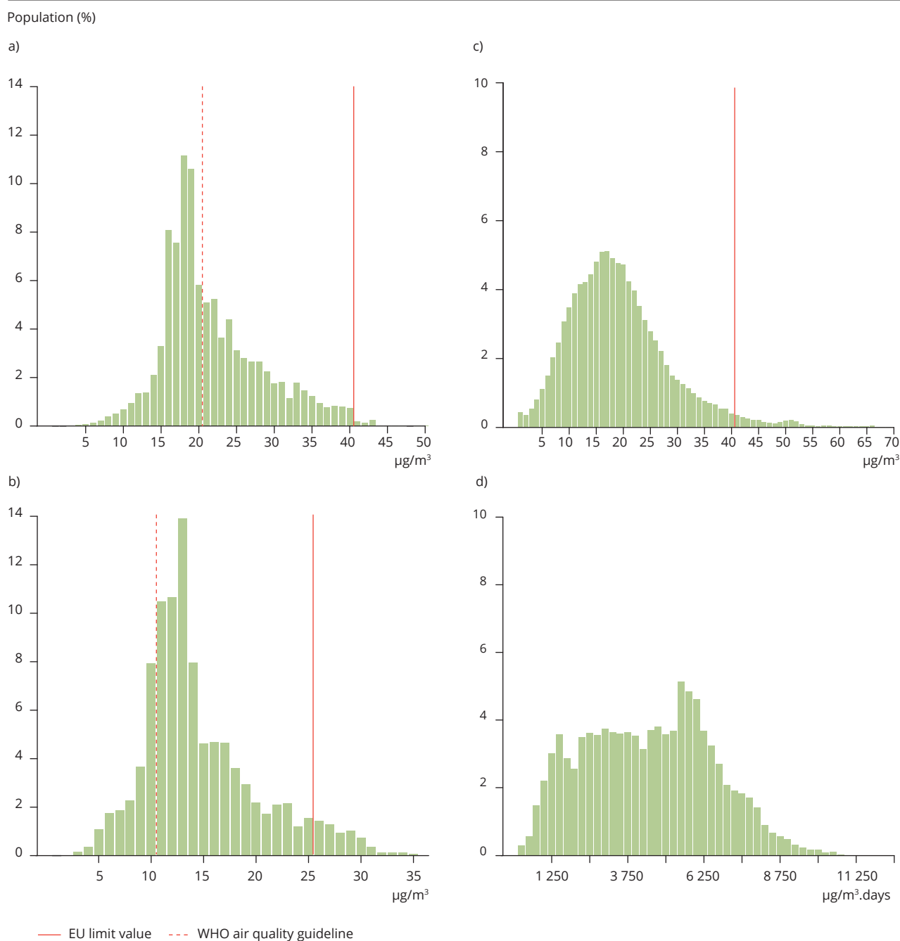
Figure 9.2 Frequency distribution of the total population exposure to (a) \text{PM}_{10} (annual mean), (b) \text{PM}_{2.5} (annual mean), (c) \text{NO}_2 (annual mean) and (d) \text{O}_3 (SOMO35) in 2015
