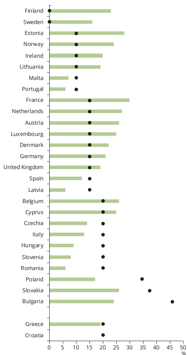
Figure 3.5 Percentage of reduction of AEI 2016 in relation to AEI 2011 and distance to the national exposure reduction target
