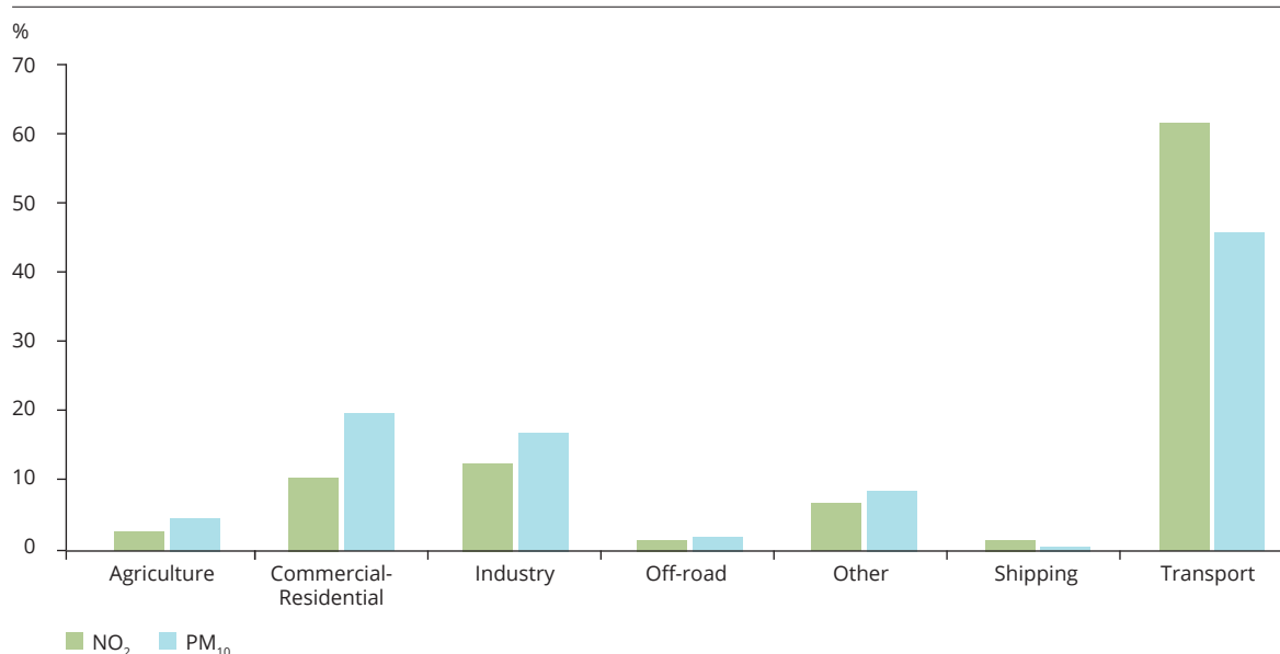
Figure 1.2 Sectors addressed by the measures reported by the EU-28 Member States for PM 10 and NO 2
