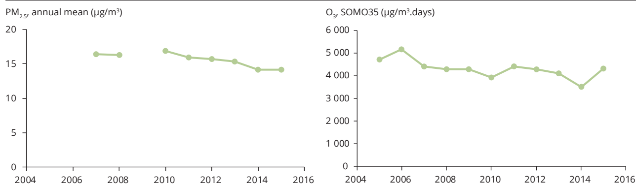
Figure 9.3 Changes in total European population exposure to \text{PM}_{2.5} (annual mean) and ozone (SOMO35)
