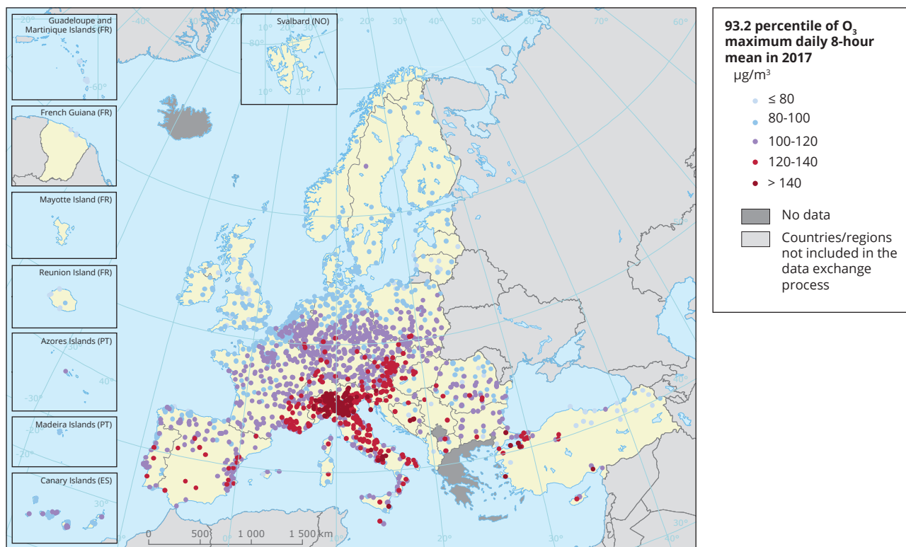
Map 4.1 Concentrations of O 3 in 2017
