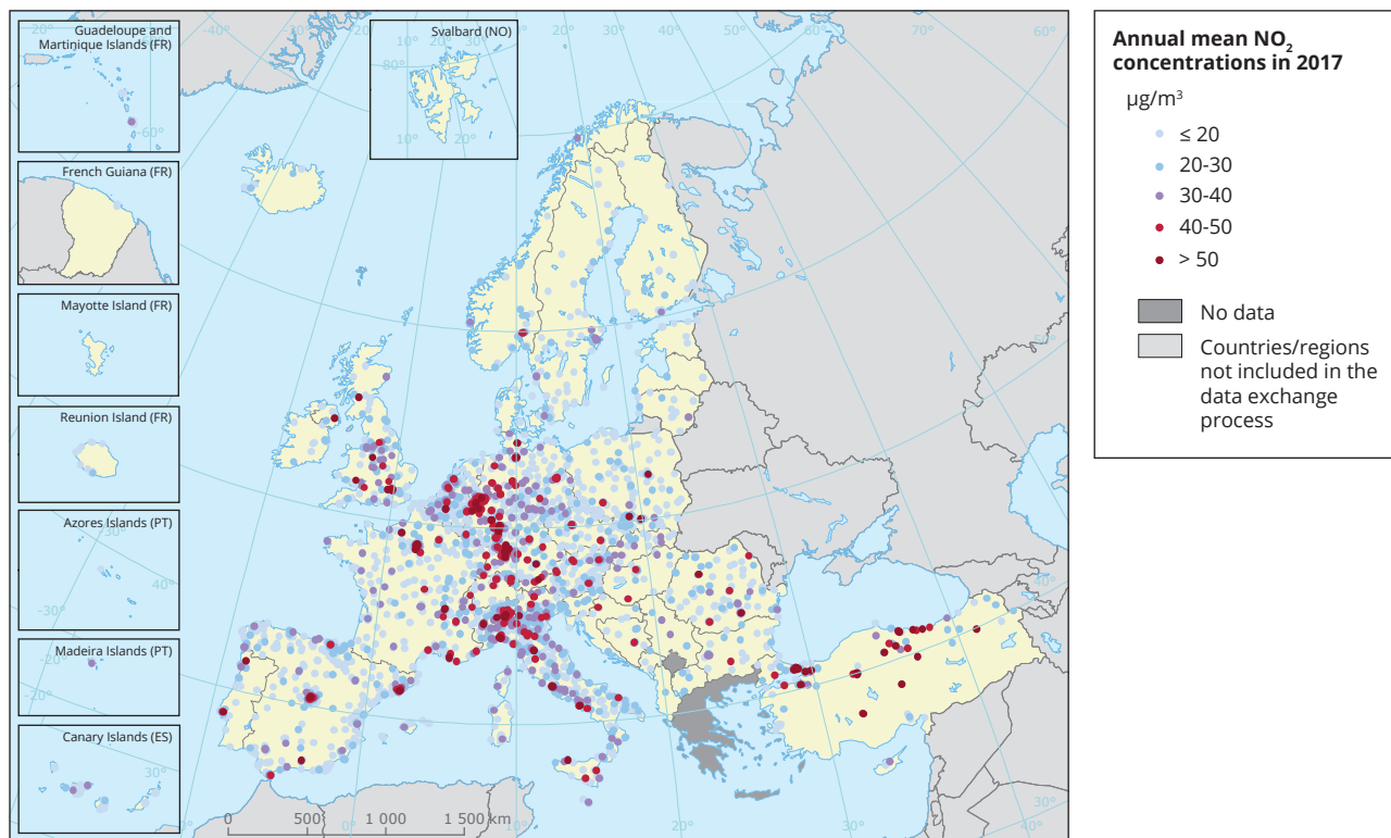
Map 5.1 Concentrations of NO 2 , 2017
