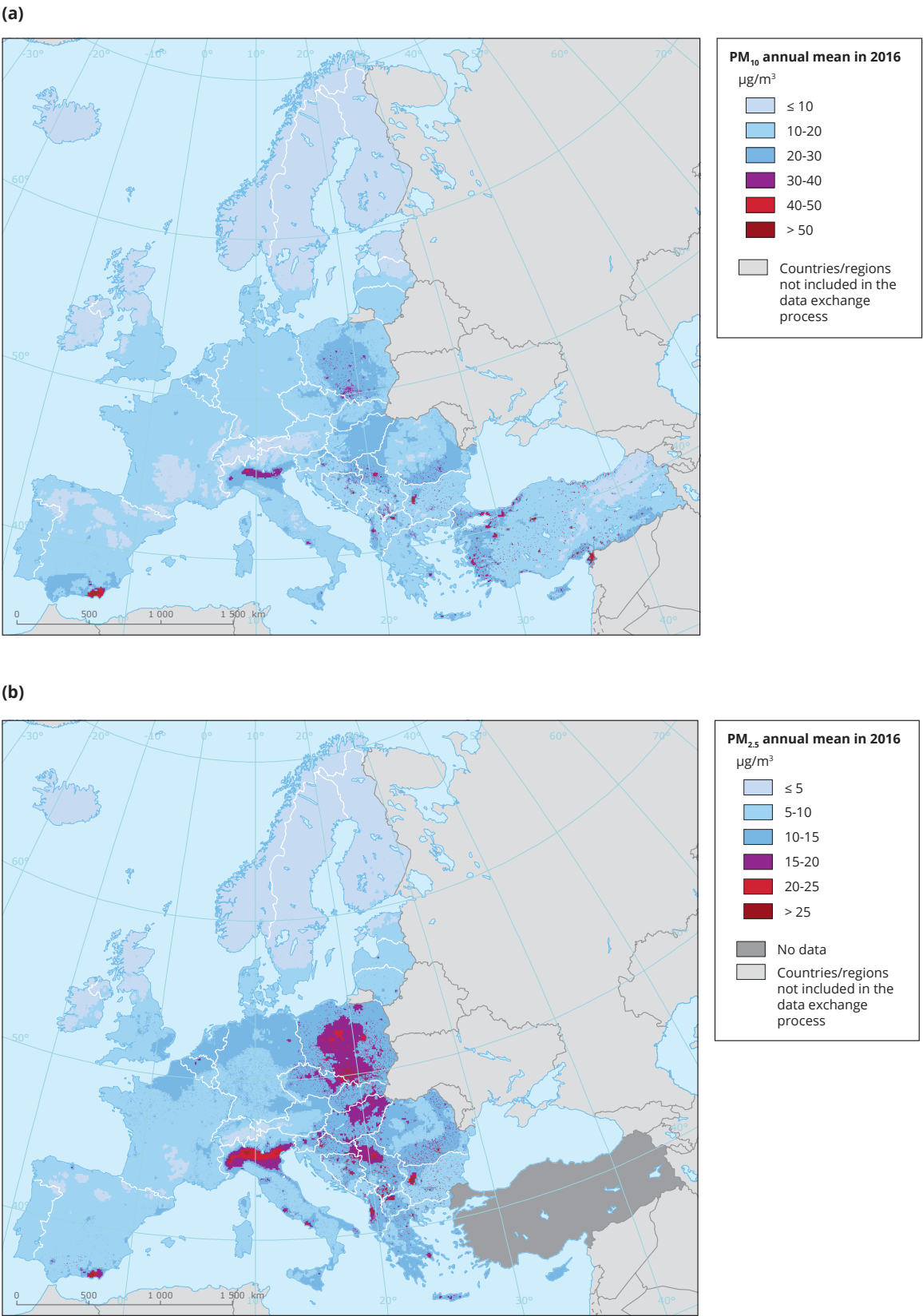
Map 9.1 Concentration interpolated maps of (a) PM 10 (annual mean, µg/m 3 ), (b) PM 2.5 (annual mean, µg/m 3 ), (c) O 3 (SOMO35, µg/m 3 ·days), and (d) NO 2 (annual mean, µg/m 3 ) for 2016
