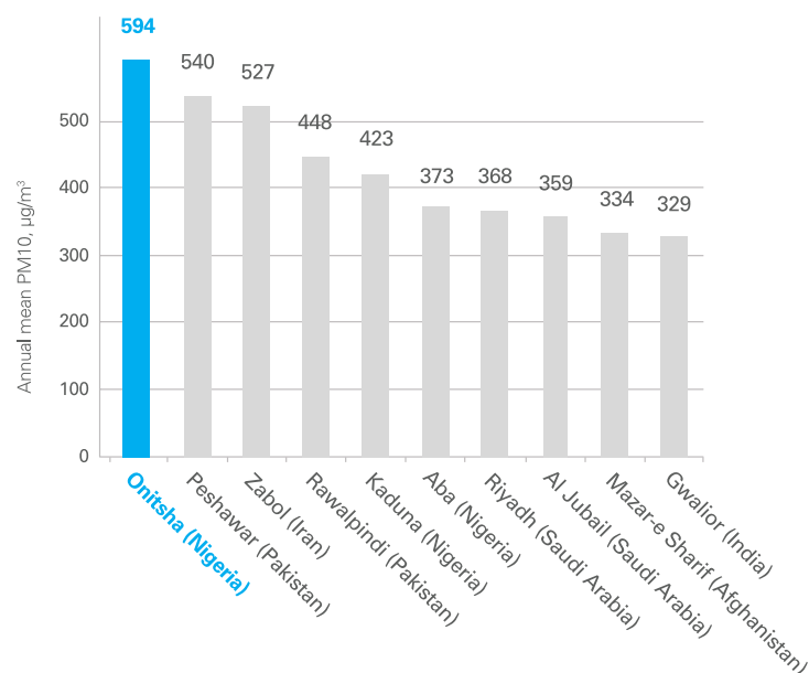
Fig. 22: Cities by PM10 pollution
