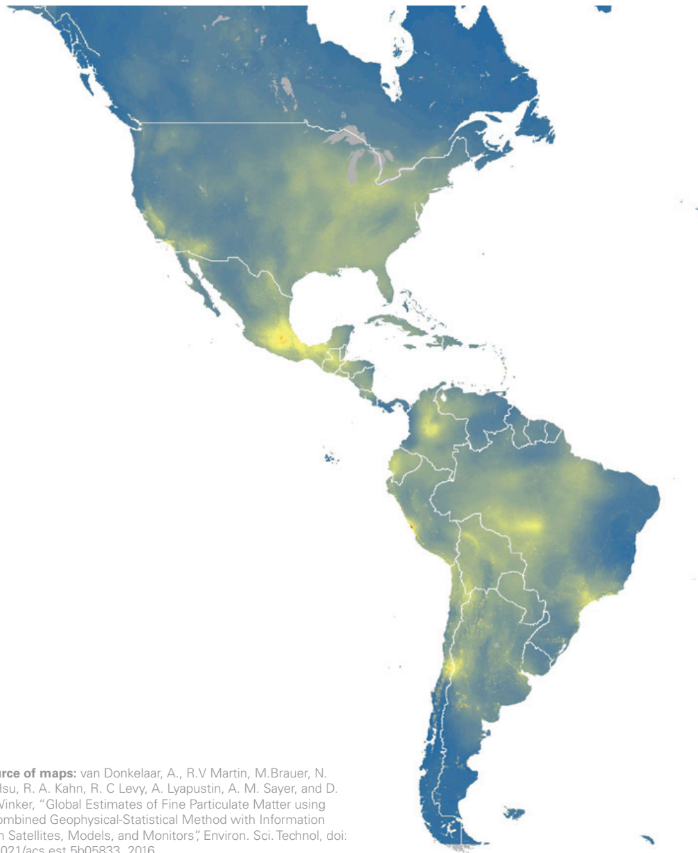
Fig. 26: Satellite derived PM 2.5 level (global annual average), Americas, 2012-2014
