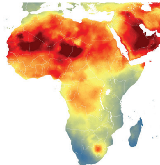
Fig. 24 Satellite derived PM 2.5 level (global annual average), Africa, 2012-2014
