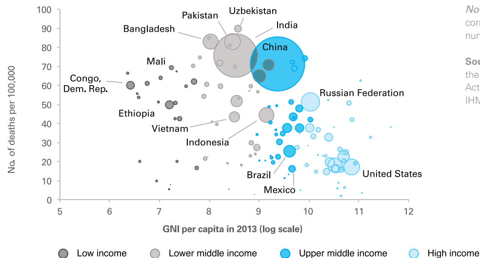
Fig. 18: Outdoor PM2.5 death rate versus income per capita, 2013
