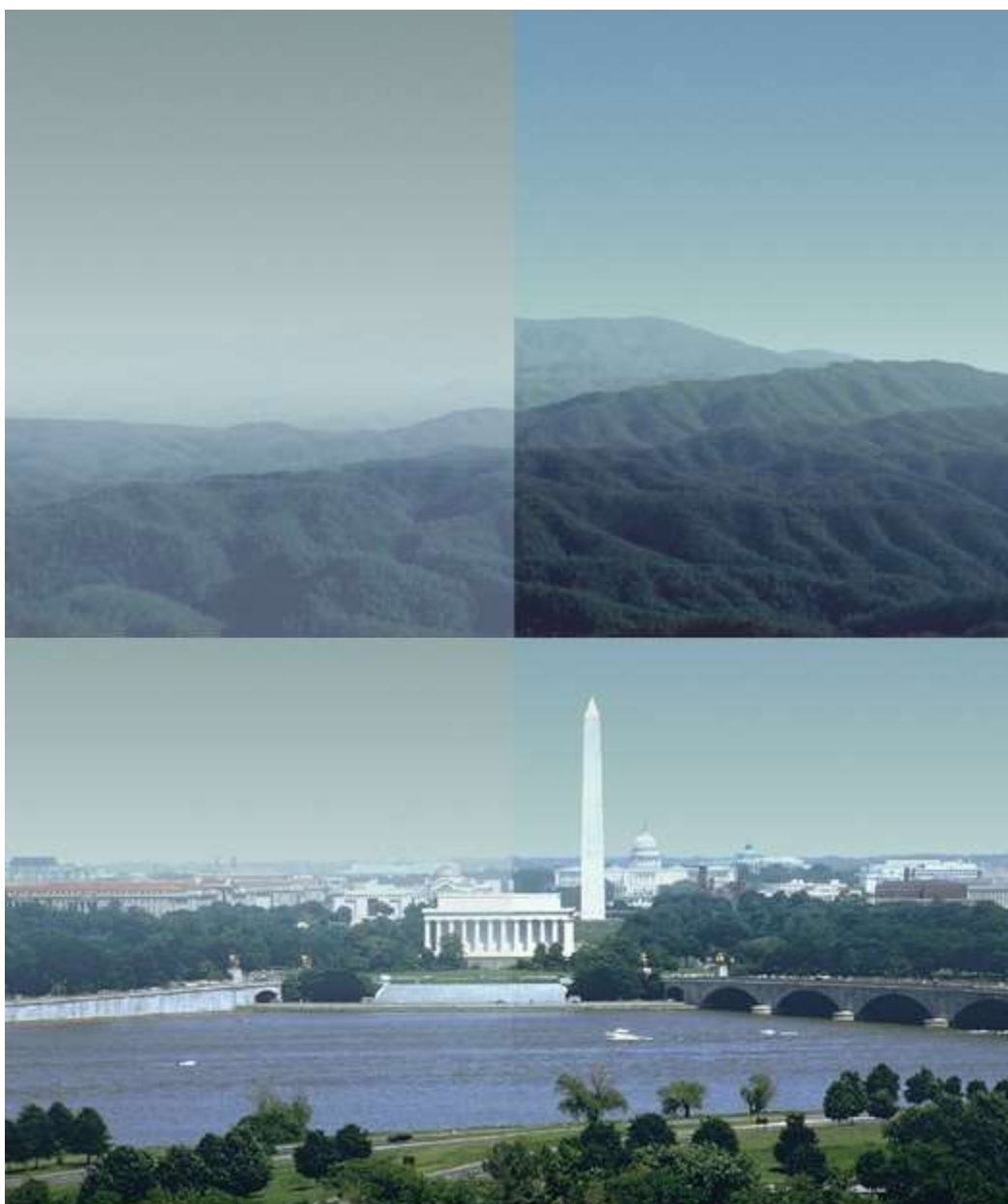
Figure 13-16 Simulations of the view at Great Smoky Mountains National Park, TN (top), and Washington, DC (bottom), corresponding to the mean 20% haziest b_{ext} in 1990 (left side of image) and 2012 (right side of image). Contributions from Rayleigh scattering are included.
