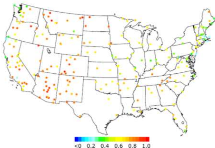
Figure 3-24 Map illustrating national-scale variability of Pearson correlation coefficients for comparison of seasonal 24-hour average total PM 10-2.5 mass concentration with mass concentration of Si in PM 10-2.5 from the Air Quality System during 2013–2015.
